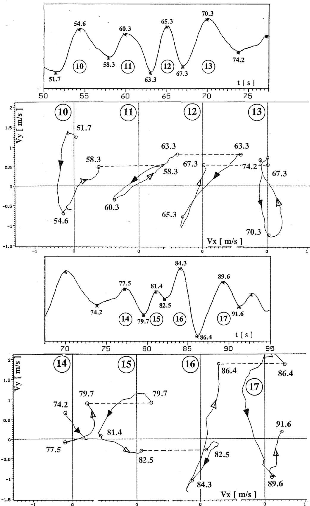
Fig. 5 b Surface elevation and velocity vector course of consecutive waves
