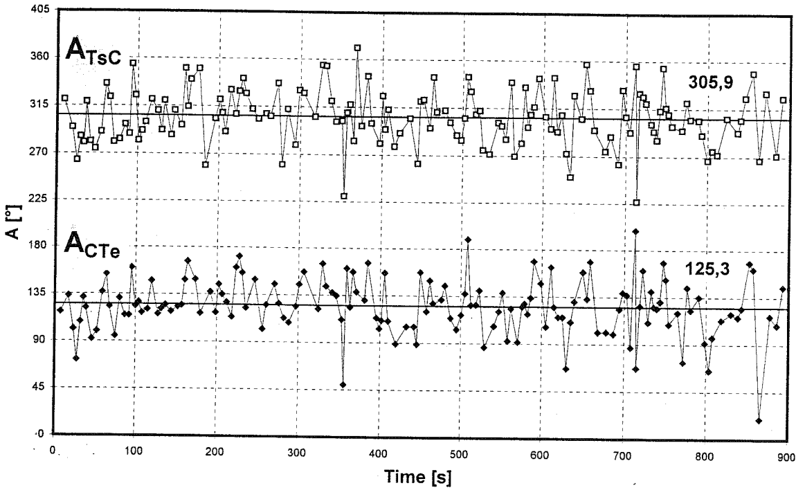
Fig. 9 Fluctuations of A_{TSC} and A_{CTe} during a period of 15 minutes
