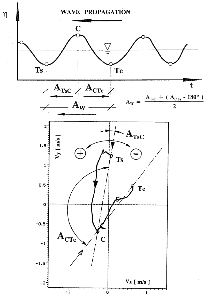
Fig. 6 Definitions for wave approach directions
