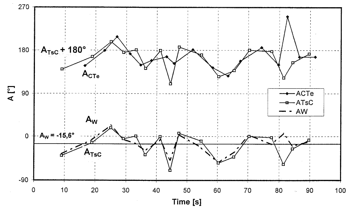
Fig. 8 Wave approach directions evaluated from the waves in Figs. 5a and 5b
