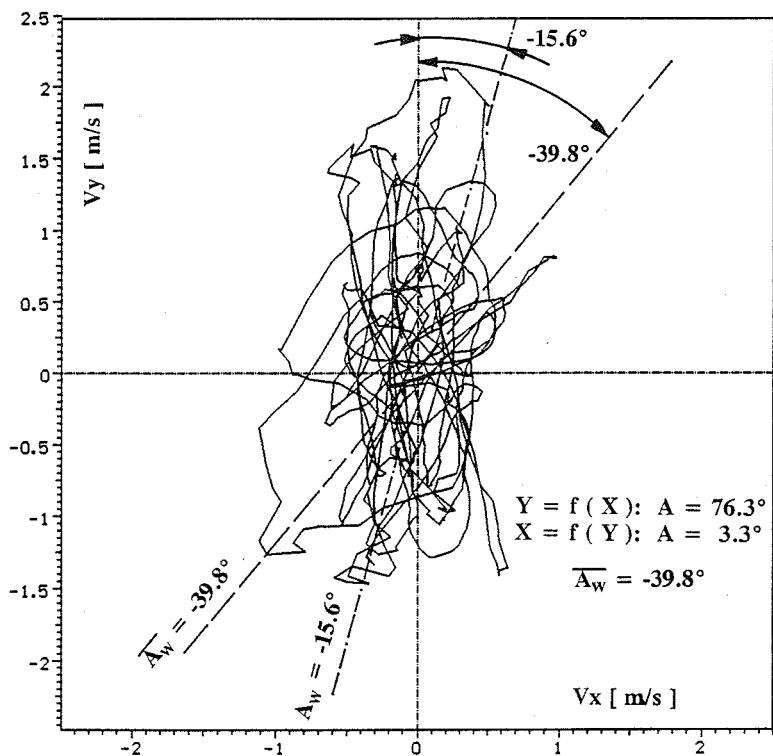
Fig. 4 Velocity vector course of velocity data S1X and S1Y from Fig. 3
