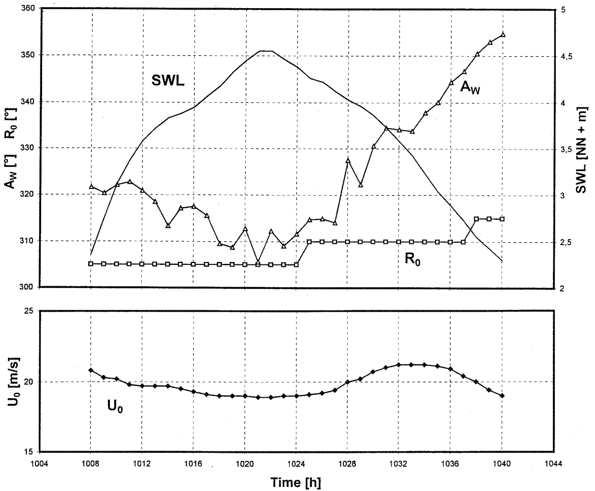
Fig. 12 Time histories of stillwaterlevel SWL, local winddirection R_0 , local windvelocity U_0 and wave approach directions A_w during a storm surge
