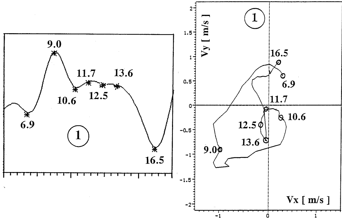
Fig. 7 Example of a wave with complex velocity vector course
