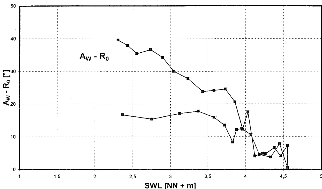
Fig. 13 Phaseshift between wave approach directions A_W and winddirection R_0
