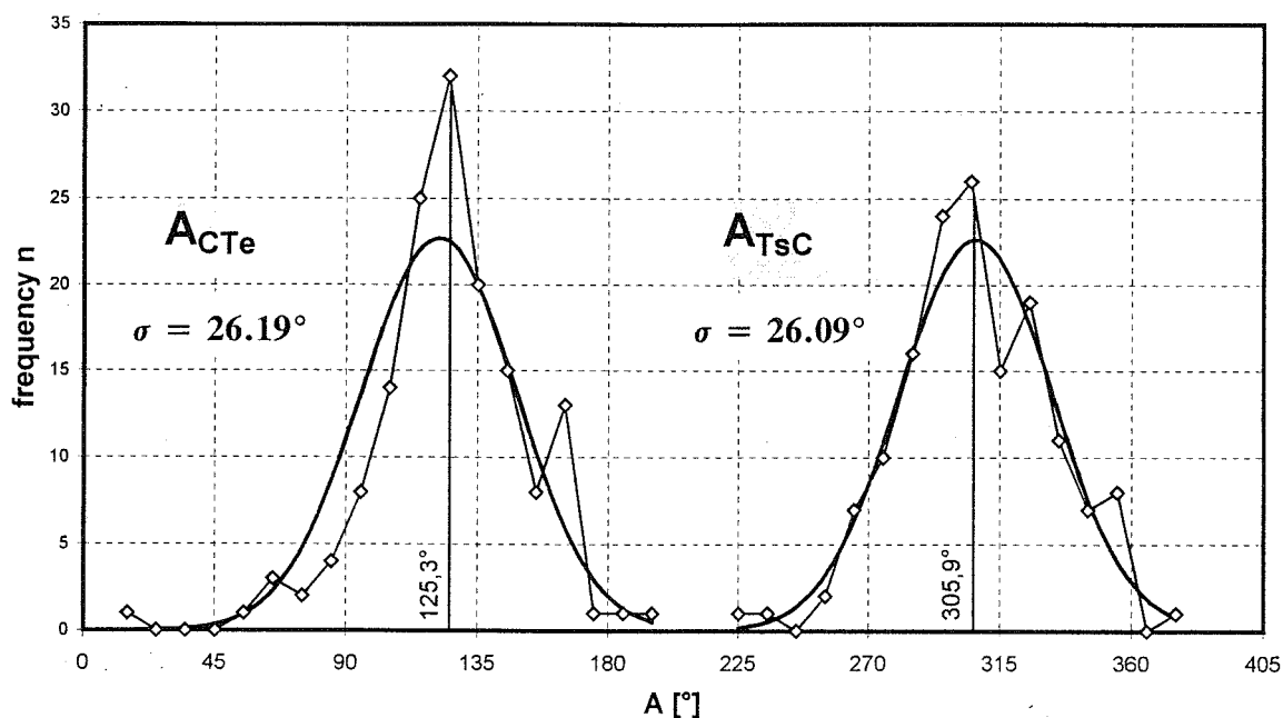
Fig. 10 Frequency distributions of A_{TsC} and A_{CTe} from the data in Fig. 9
