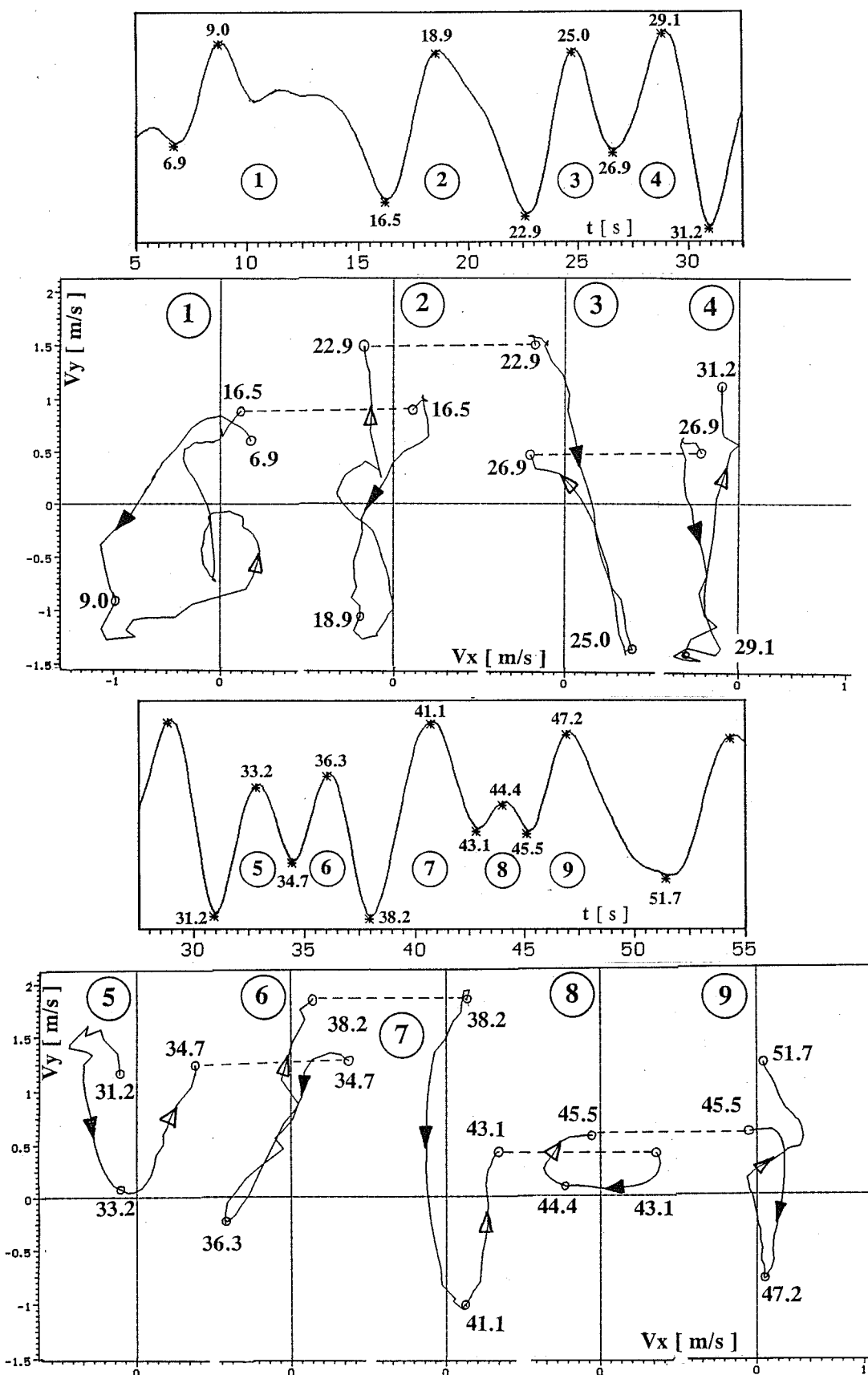
Fig. 5 a Surface elevation and velocity vector course of consecutive waves
