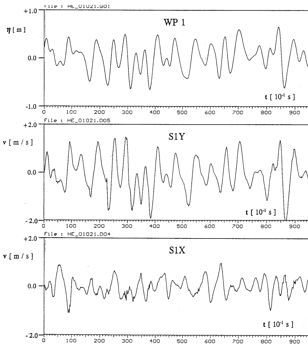
Fig. 3 Example of synchronously recorded wave and velocity data
