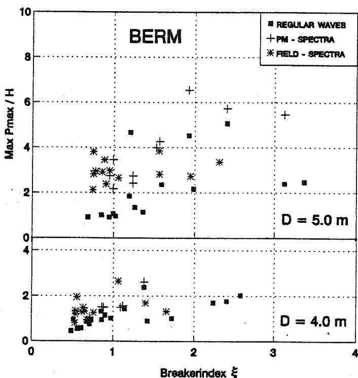
Fig. 9 \text{Max } P_{\text{max}}/H versus breakerindex \xi for different wave characteristics
