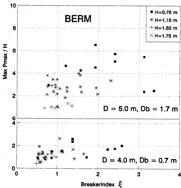
Fig. 7 Max Pmax/H versus breakerindex \xi for of regular and irregular waves
