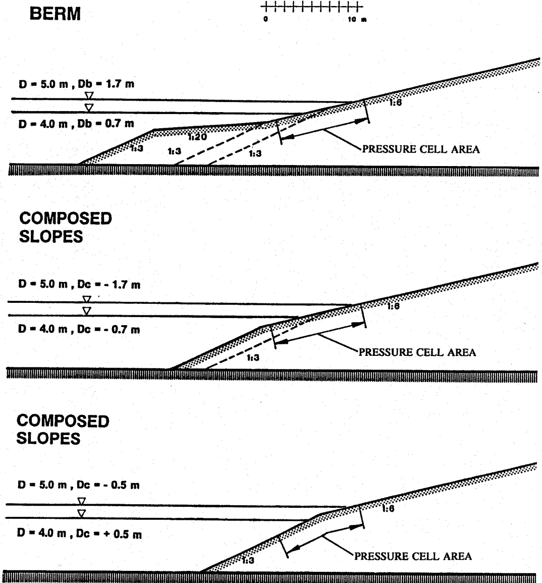
Fig. 1 Dyke cross-sections with berm and composed slopes, investigated in the LARGE WAVE CHANNEL (GWK)
