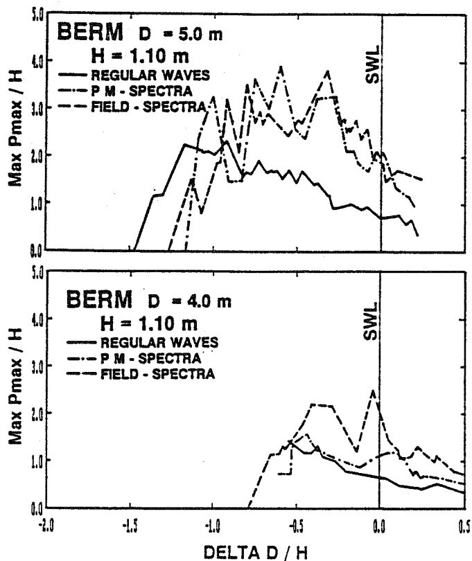
Fig. 8 Local distribution of \text{Max } P_{\text{max}}/H for different wave characteristics
