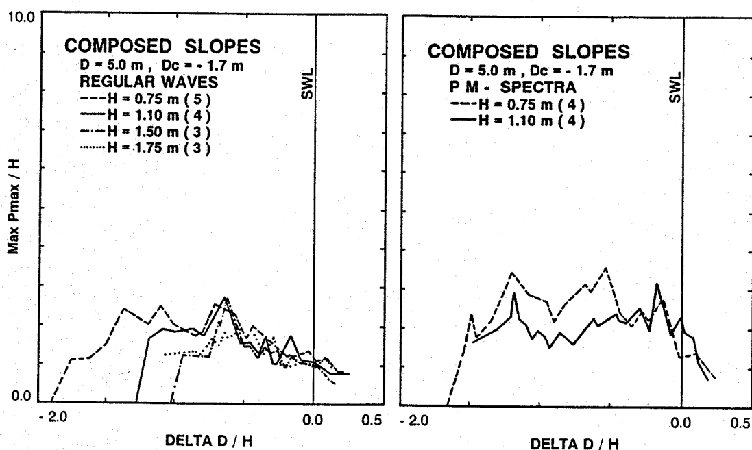
Fig. 11 Local distribution of Max P_{max}/H for testseries with regular waves.
