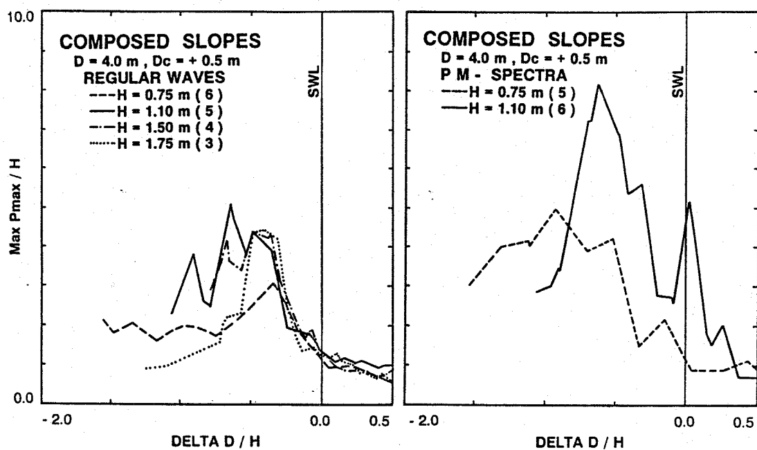
Fig. 13 Local distribution of Max P_{max}/H for regular waves and PM - spectra
