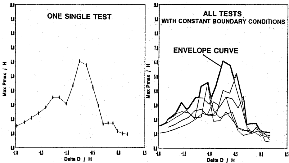
Fig. 4 Example for a local distribution of pressure data \text{Max } P_{\text{max}}/H
