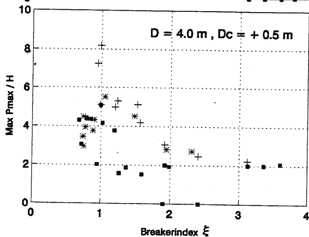
Fig. 14 Max P_{max}/H versus breakerindex \xi for all testseries with composed slopes
