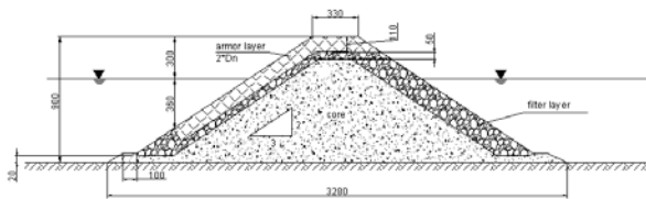
Figure 1: Cross-section of installed breakwater (model values in [mm])
