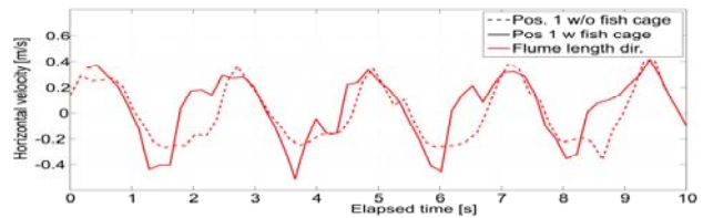
Figure 4. Horizontal velocity from PIV-measurements comparing setup with and without fish cages assembled
