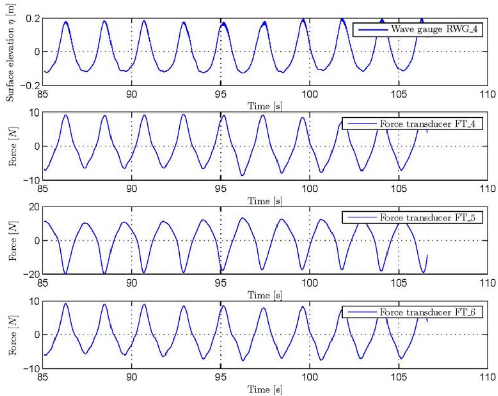
Figure 5. Time series of water surface elevation and forces for a representative period of the wave train, one net layer
