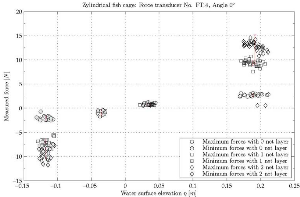
Figure 6. Correlation of maximum wave heights and measured forces for cylindrical fish cages for force transducer FT_4 with respect to the number of net layers
