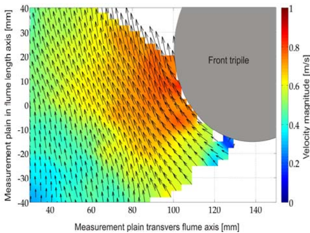
Figure 4. Horizontal velocity from PIV-measurements comparing setup with and without fish cages assembled
