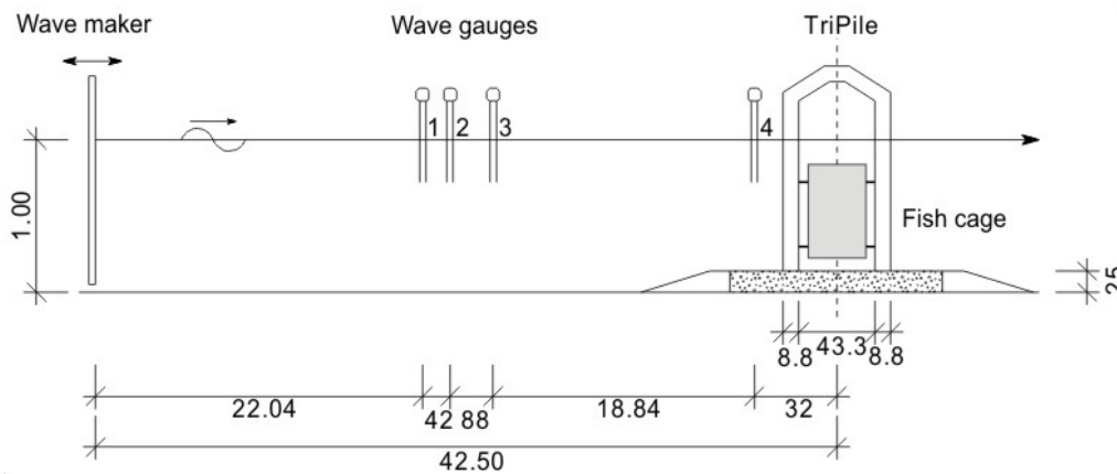
Figure 2. Schematic experimental setup with wave maker, instrumentation and the tripile position
