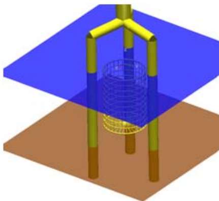
Figure 1. Schematic overview of the co-use of aquaculture fish cage and offshore wind energy converter structure (Institute for Steel Construction, Hannover)
